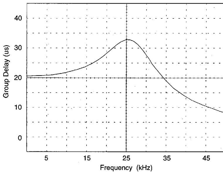
Figure 19. Simulated Analog Filter Group Delay
