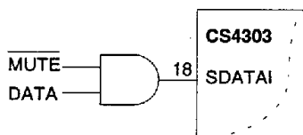
Figure 12. Muting Implementation
