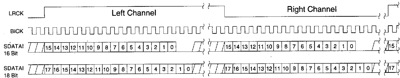
Figure 9. Digital Input Format 2
