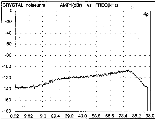
Figure 20. Unmuted Noise
