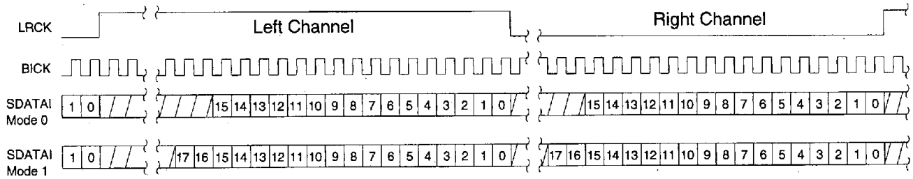
Figure 8. Digital Input Formats 0 & 1
