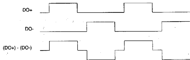
Figure 6. CS4303 Differential Outputs
